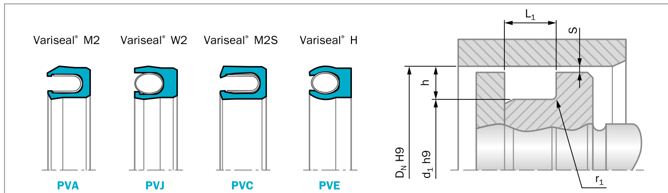
Figure 22: Installation drawing
