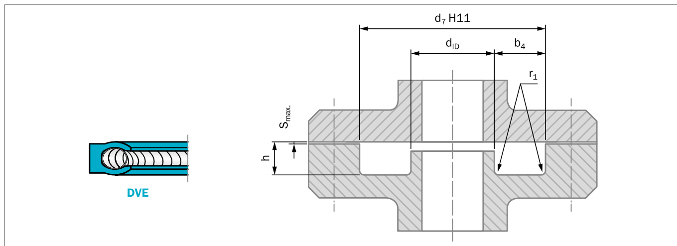
Figure 25: Installation drawing
