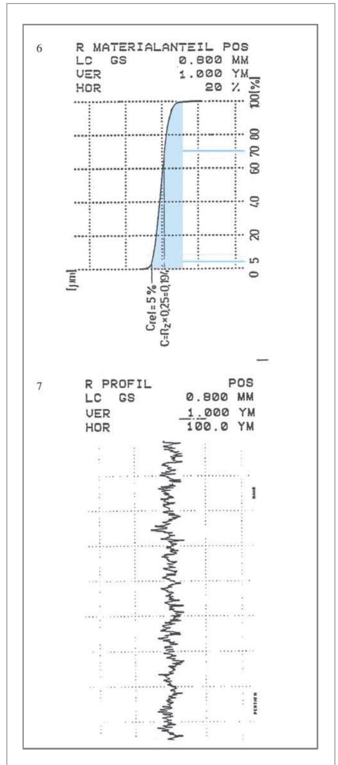
Figure 13: Measurement printout
