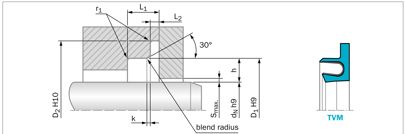
Figure 31: Installation drawing
